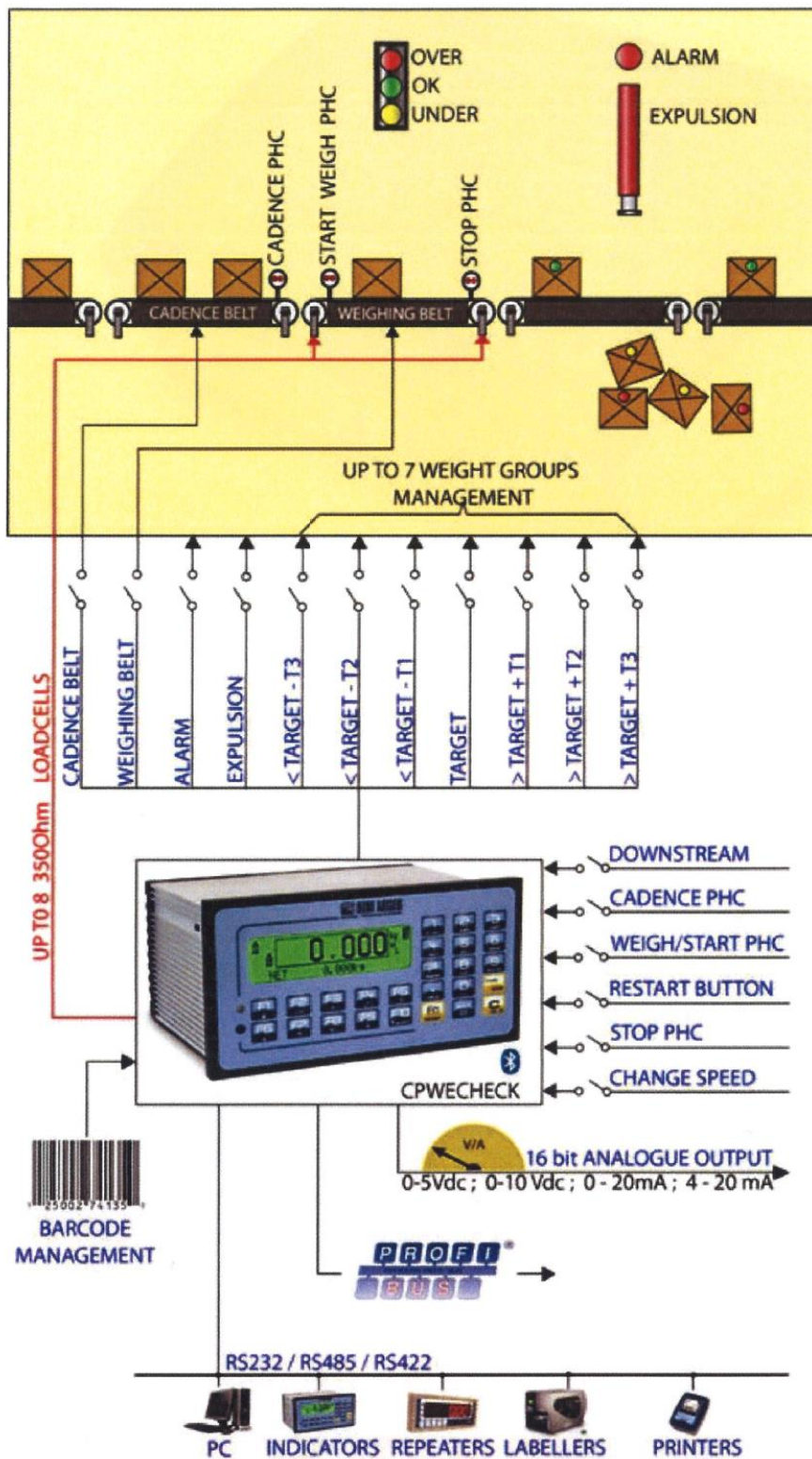
Figure 1 Typical configuration
