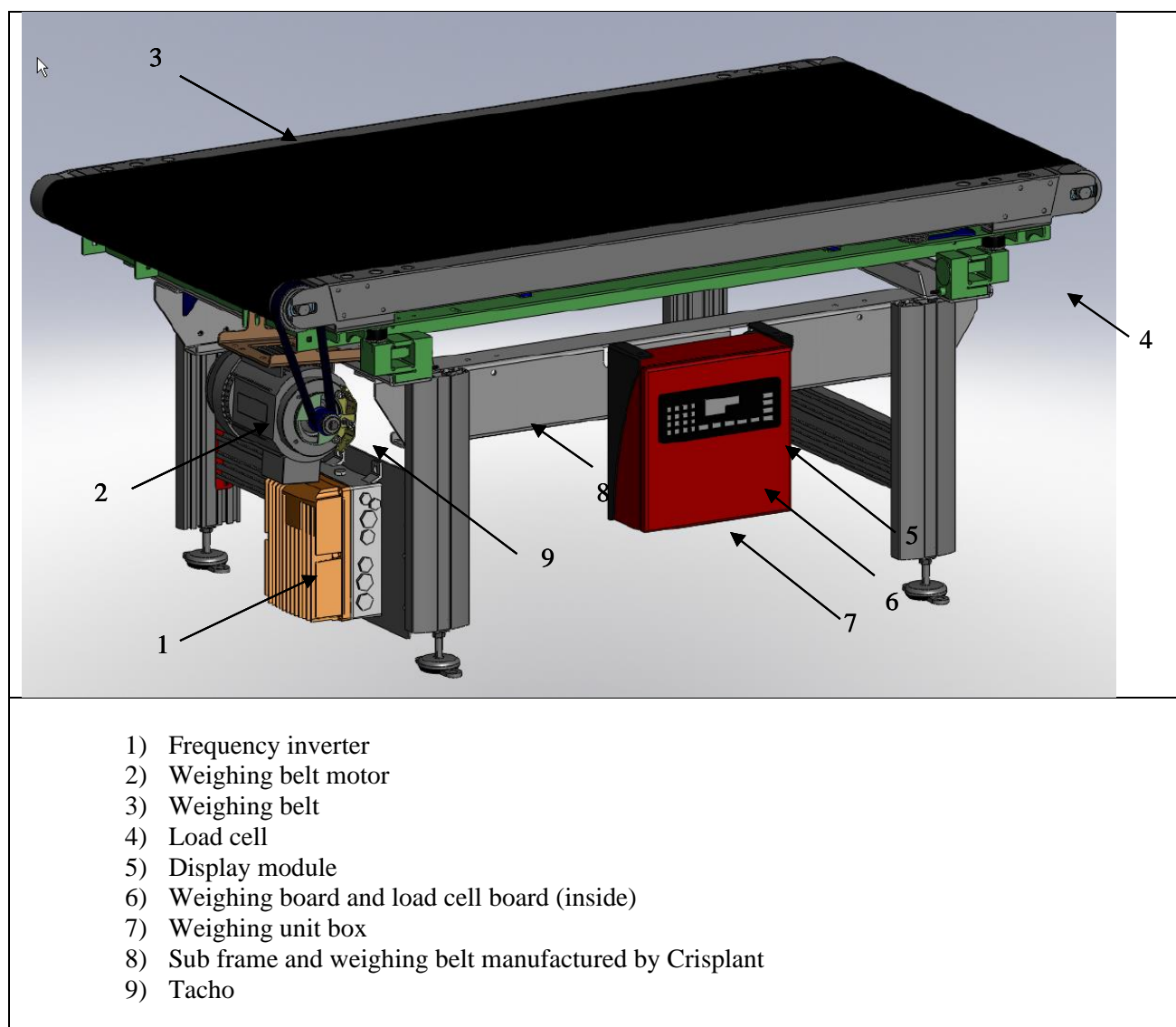
Figure 1 Mechanical Construction
