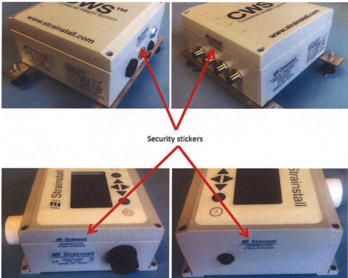
Figure 7 Enclosure sealing method (Interface and Display units)
