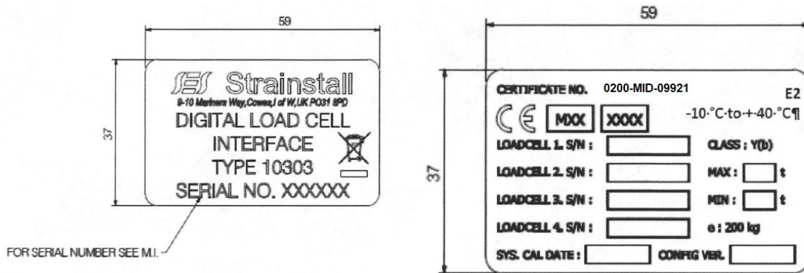
Figure 5 Rating plate example (Interface unit)
