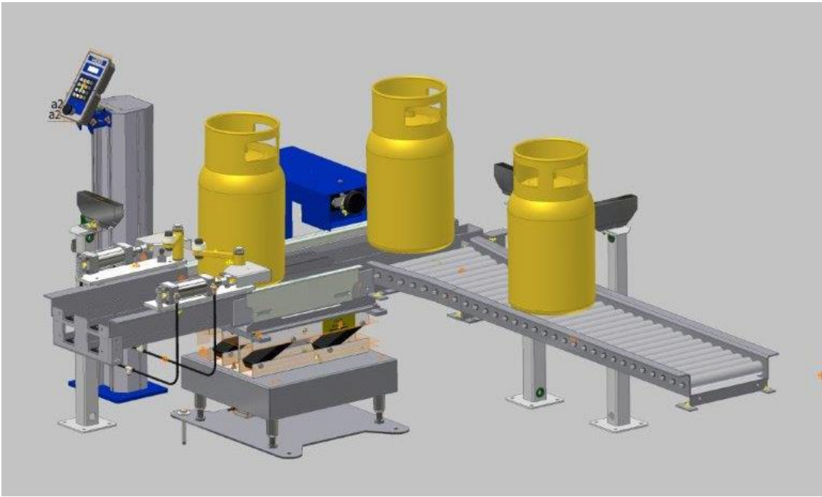
Figure 3 ECS Check Weighing with static lifting table
